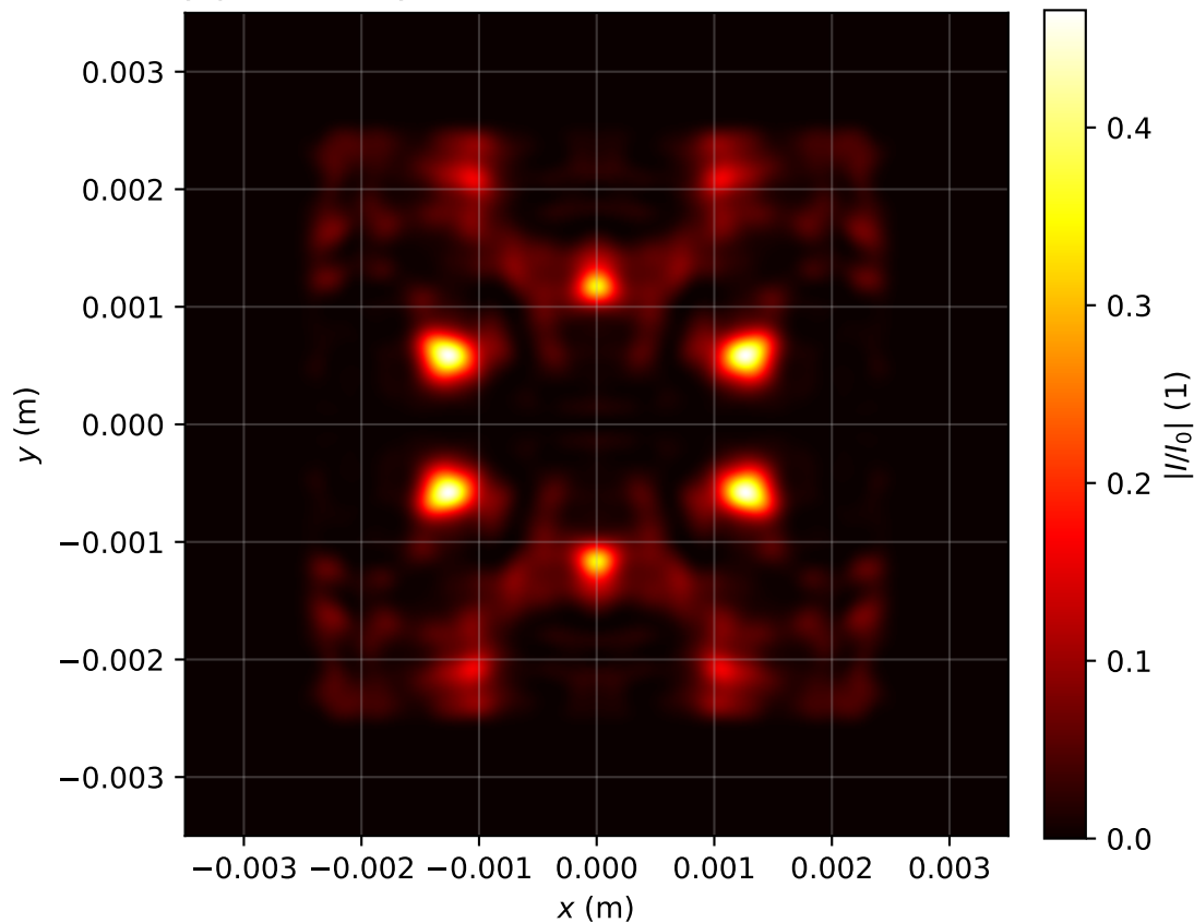
Intensity profile I(x, y, z = 3.264)/I_0 , P_{in}=20.0\text{Pcr} , artificial time
