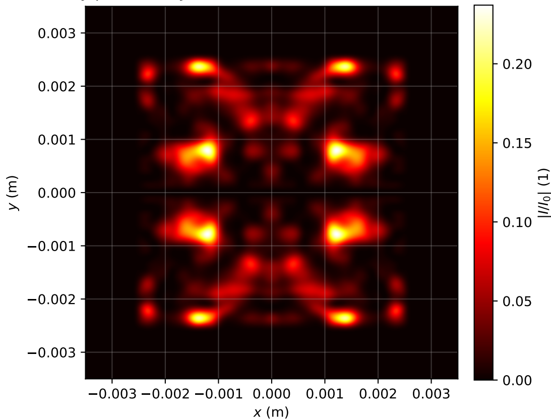
Intensity profile I(x, y, z = 3.901)/I_0 , P_{in}=20.0\text{Pcr} , artificial time
