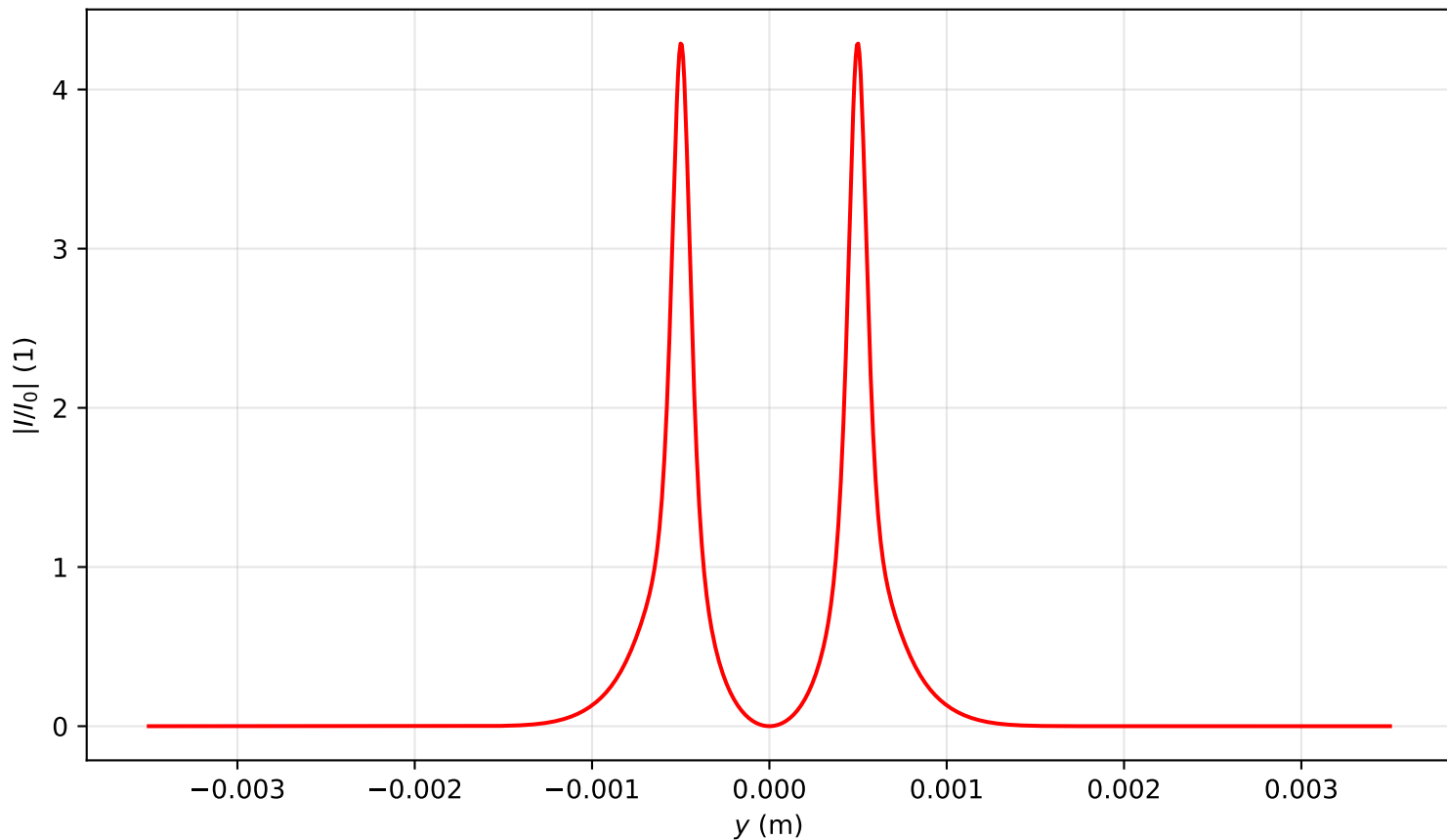
Intensity profile I(x = 0, y, z = 0.239)/I_0 , P_{in}=20.0P_{cr} , artificial time
