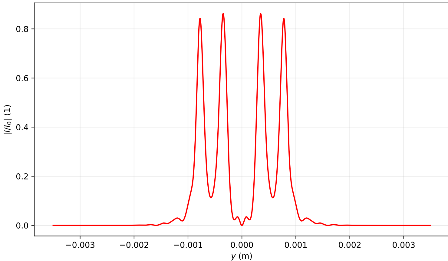
Intensity profile I(x=0, y, z=0.557)/I_0 , P_{in}=20.0P_{cr} , artificial time
