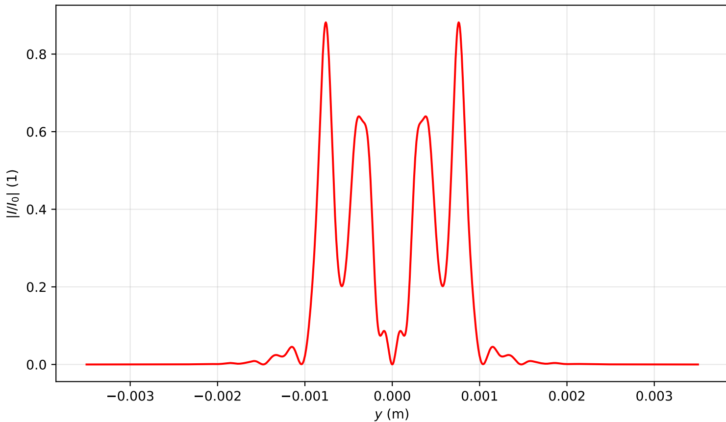
Intensity profile I(x=0, y, z=0.637)/I_0 , P_{in}=20.0\text{Pcr} , artificial time
