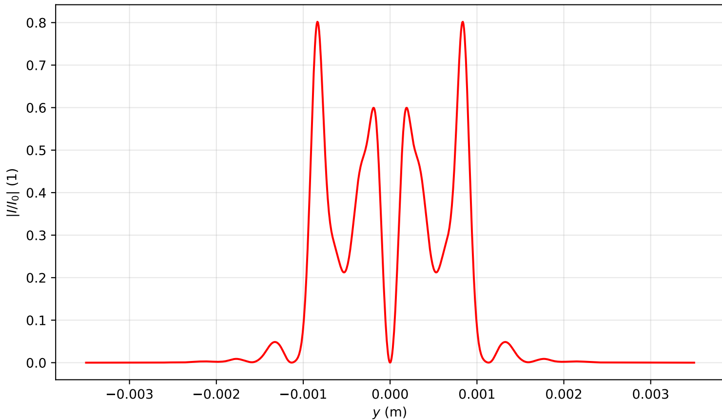
Intensity profile I(x=0, y, z=0.716)/I_0 , P_{in}=20.0\text{Pcr} , artificial time
