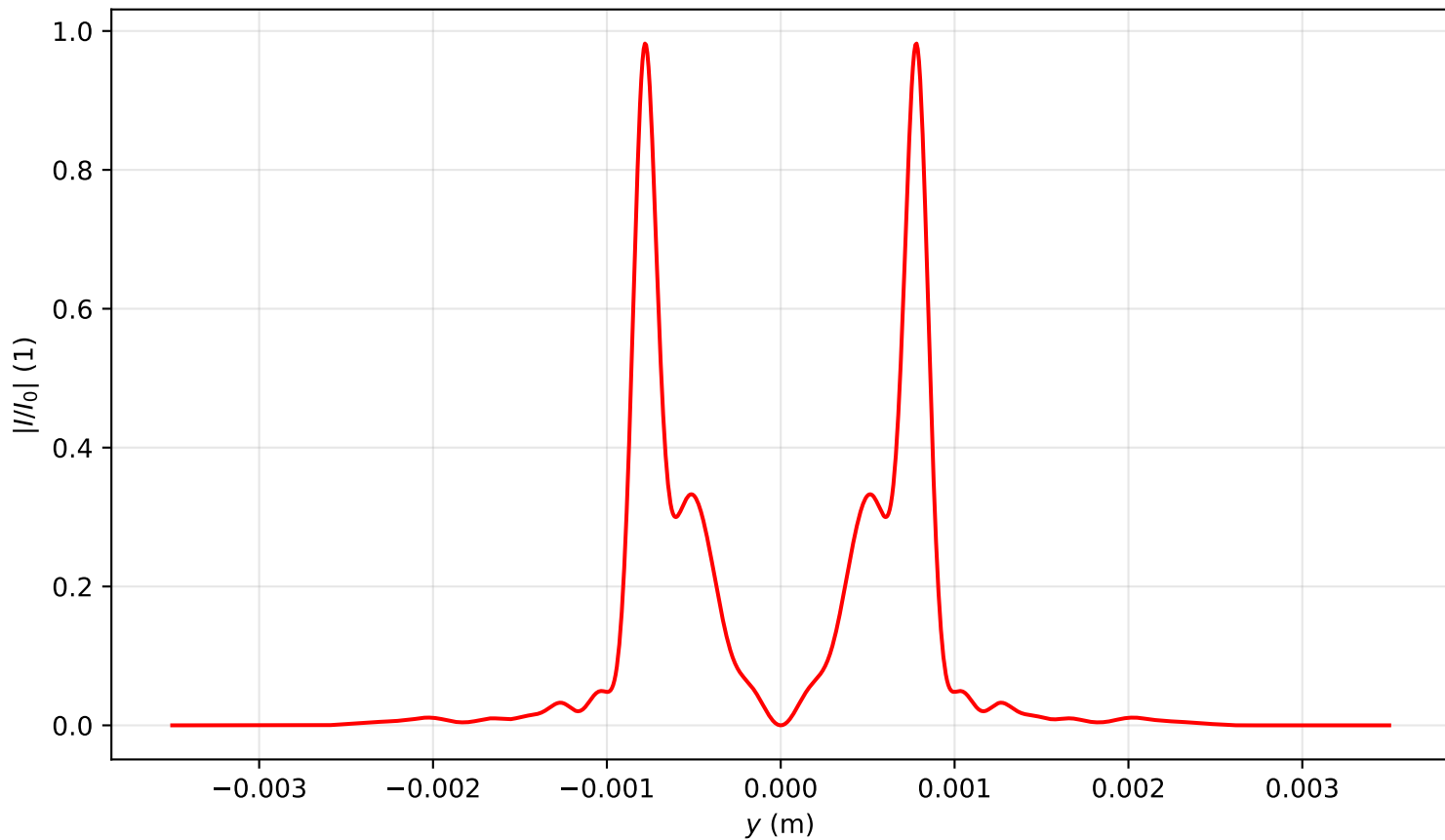
Intensity profile I(x=0, y, z=0.876)/I_0 , P_{in}=20.0\text{Pcr} , artificial time
