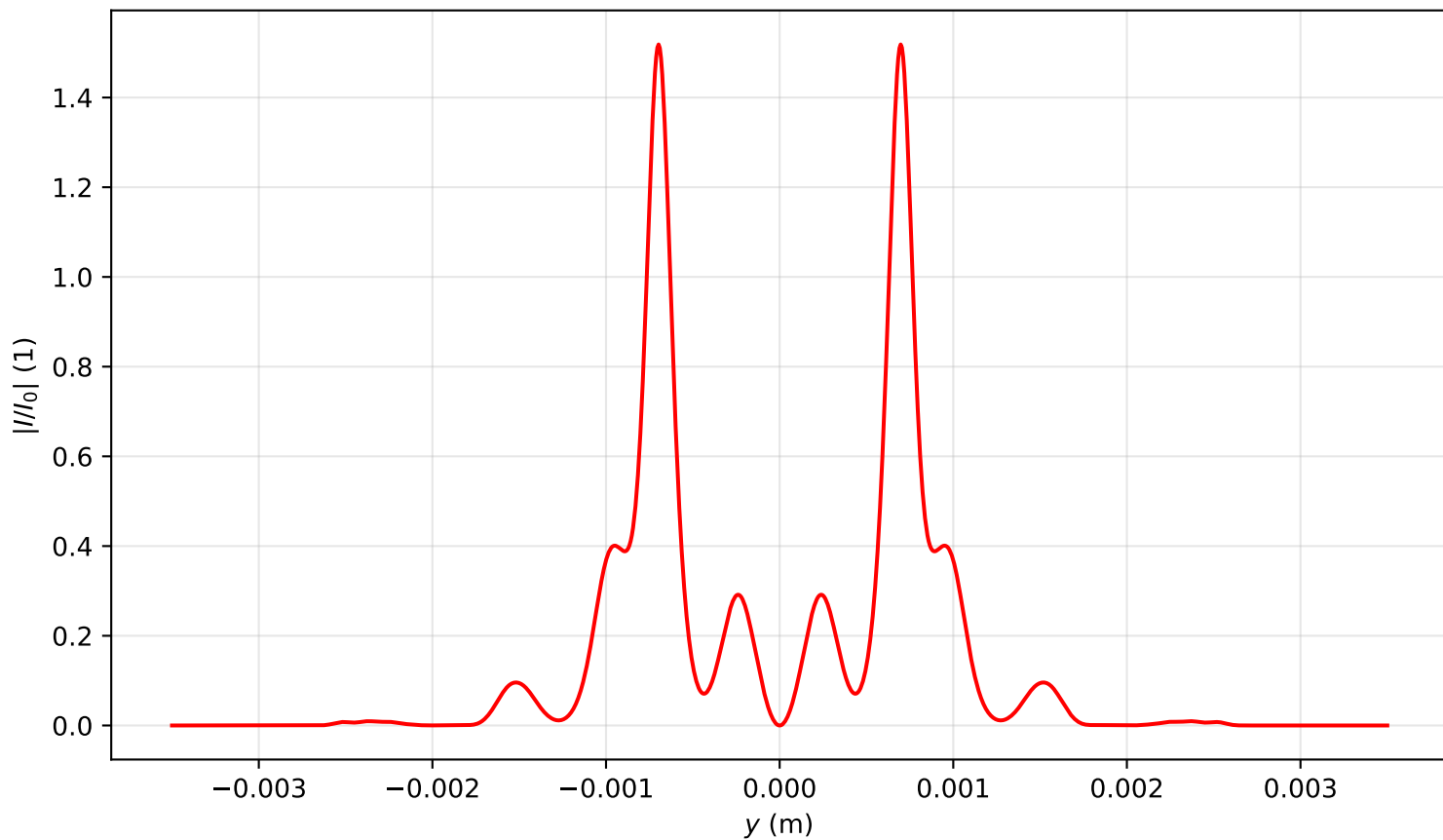
Intensity profile I(x=0, y, z=1.035)/I_0 , P_{in}=20.0P_{cr} , artificial time
