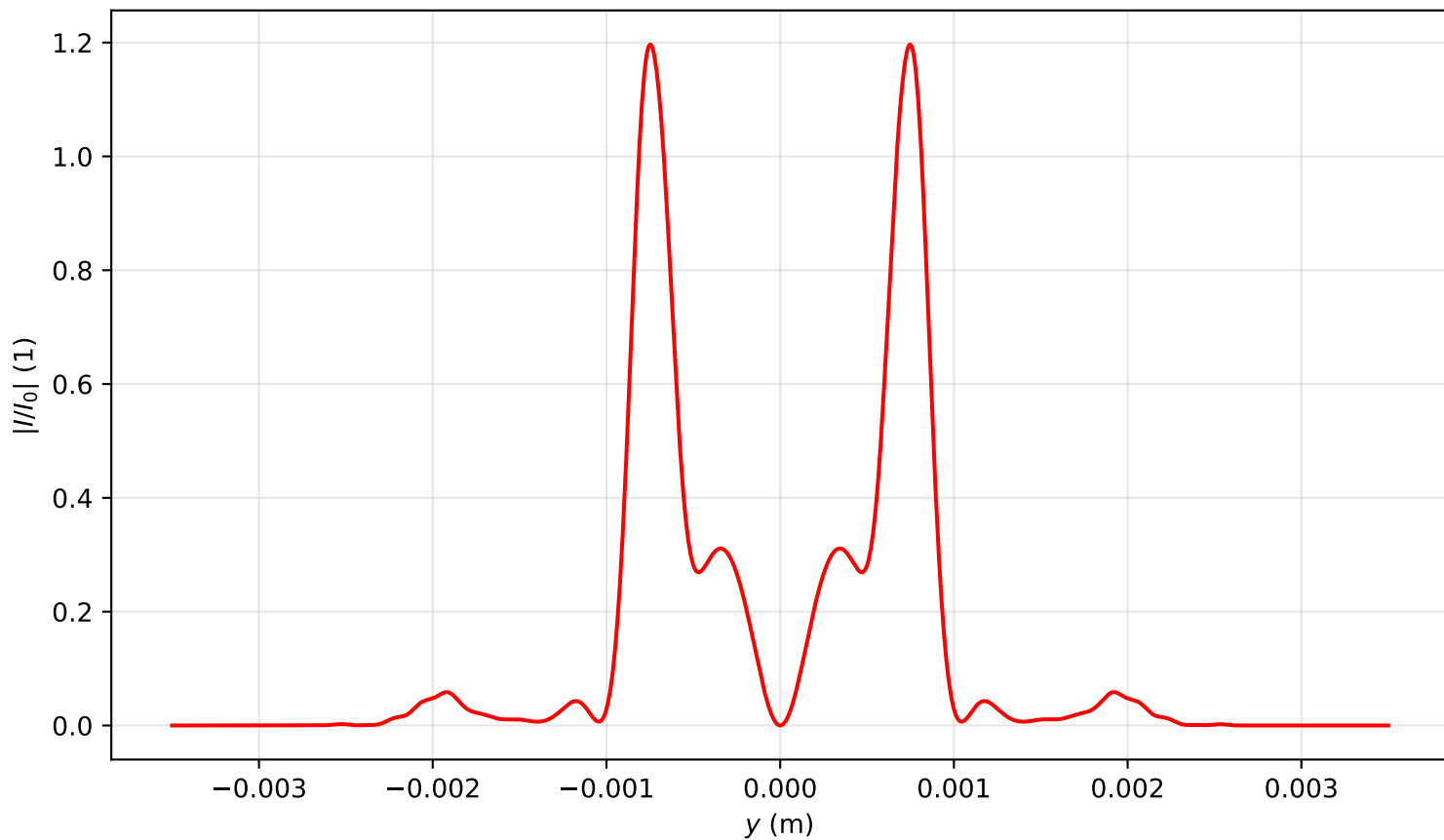
Intensity profile I(x=0, y, z=1.274)/I_0 , \text{Pin}=20.0\text{Pcr} , artificial time
