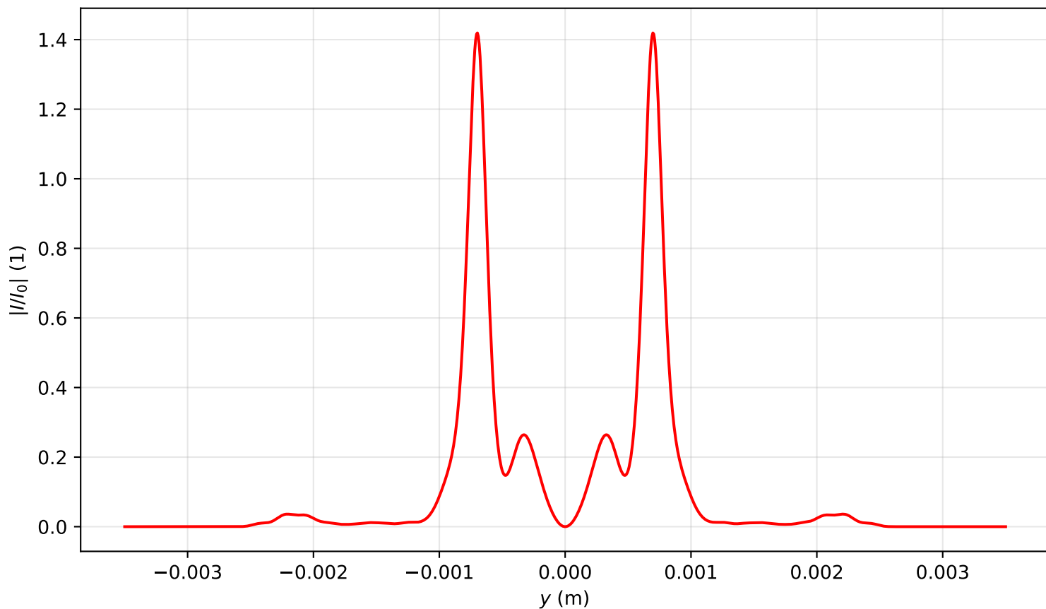
Intensity profile I(x=0, y, z=1.353)/I_0 , P_{in}=20.0P_{cr} , artificial time
