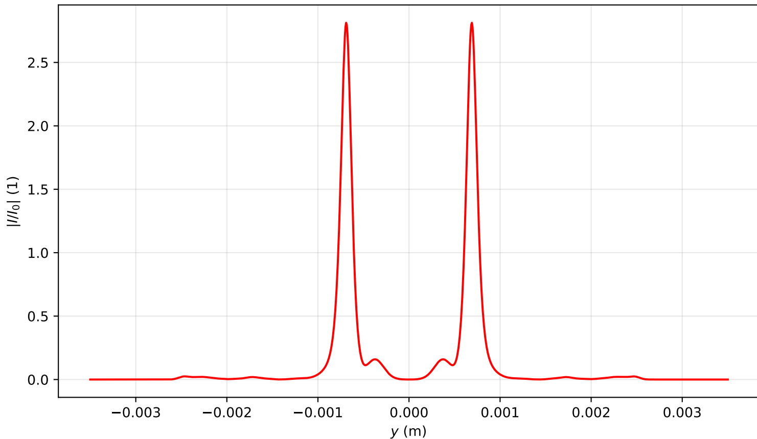
Intensity profile I(x=0, y, z=1.433)/I_0 , P_{in}=20.0P_{cr} , artificial time
