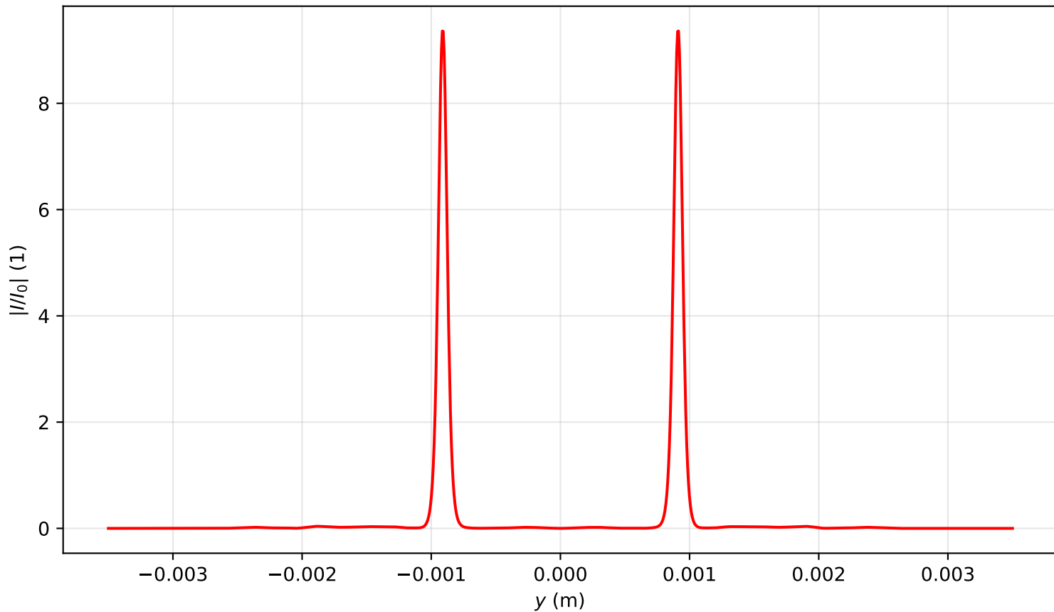
Intensity profile I(x=0, y, z=2.627)/I_0 , P_{in}=20.0P_{cr} , artificial time
