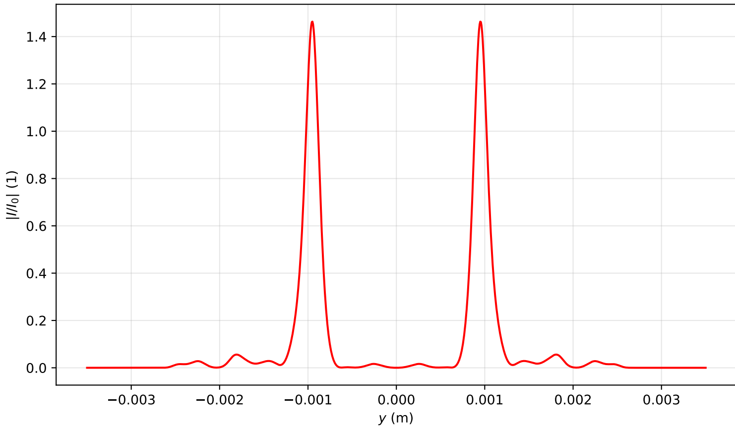
Intensity profile I(x=0, y, z=2.786)/I_0 , P_{in}=20.0\text{Pcr} , artificial time
