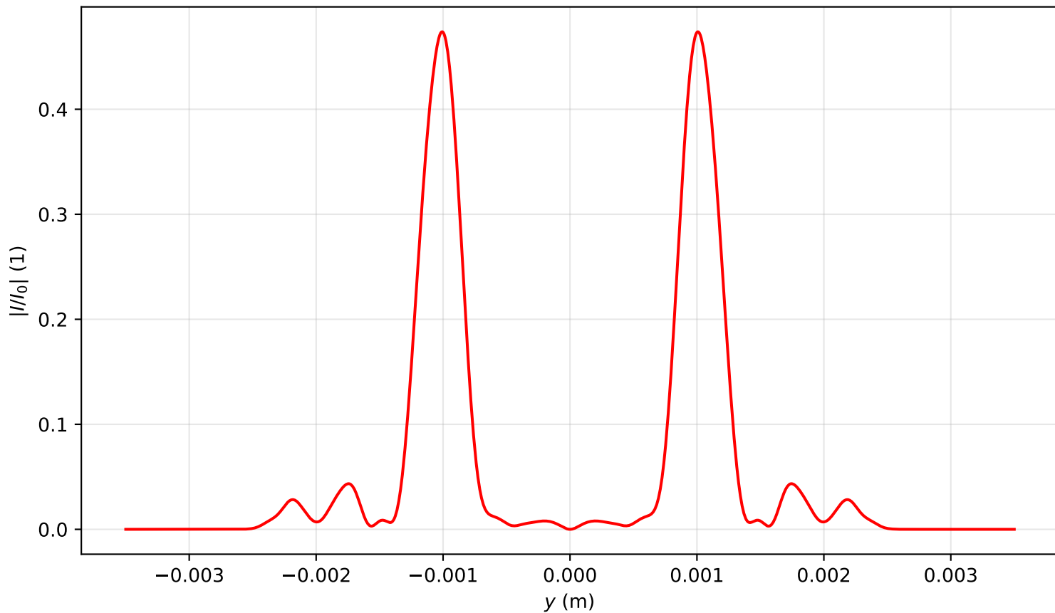
Intensity profile I(x=0, y, z=2.946)/I_0 , P_{in}=20.0P_{cr} , artificial time
