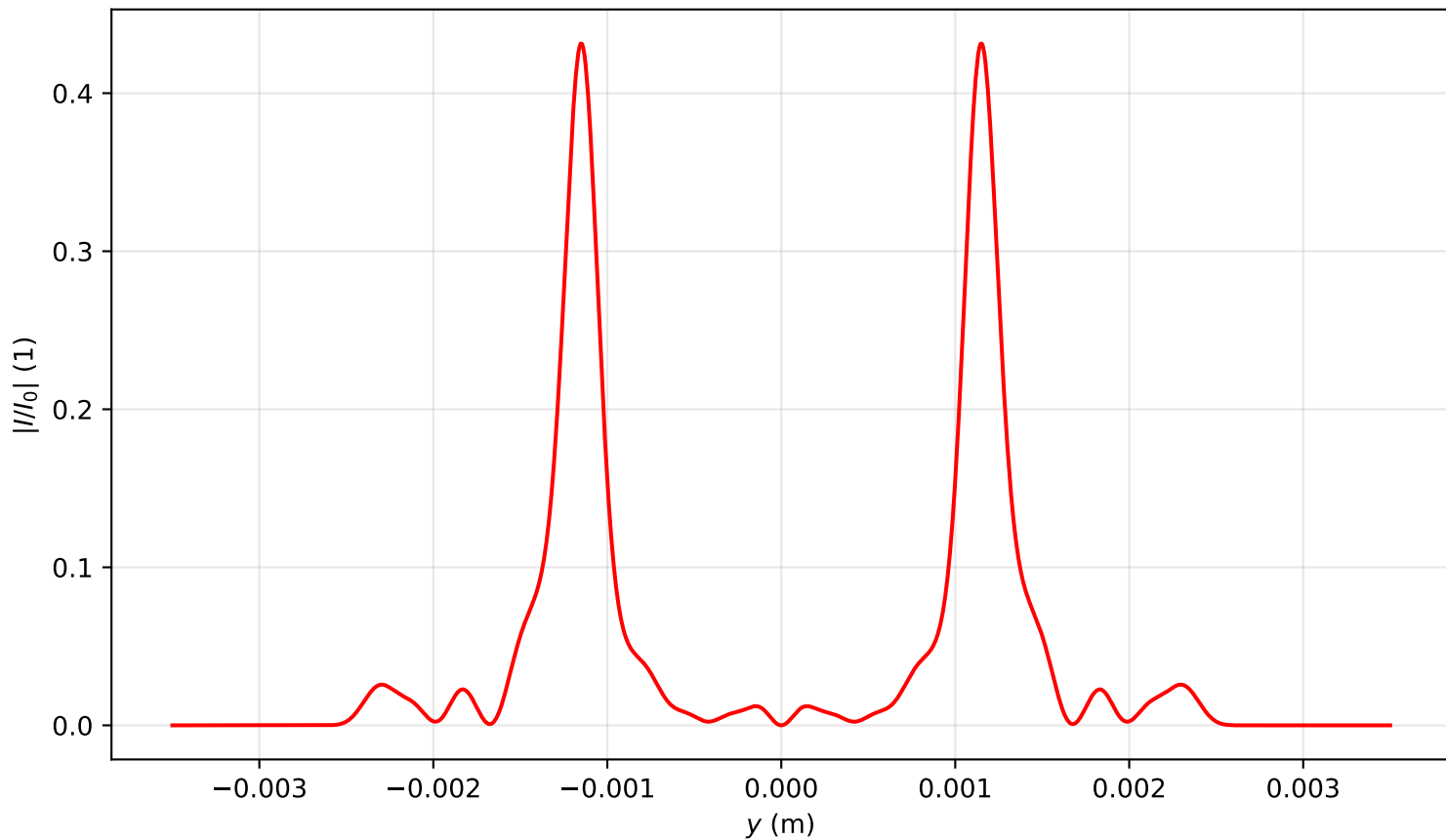
Intensity profile I(x=0, y, z=3.184)/I_0 , P_{in}=20.0P_{cr} , artificial time
