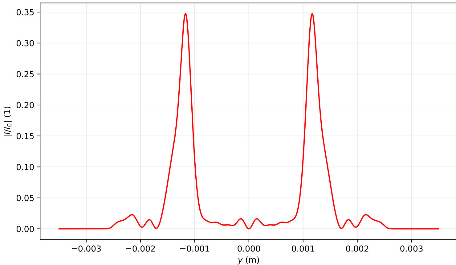
Intensity profile I(x=0, y, z=3.264)/I_0 , P_{in}=20.0P_{cr} , artificial time
