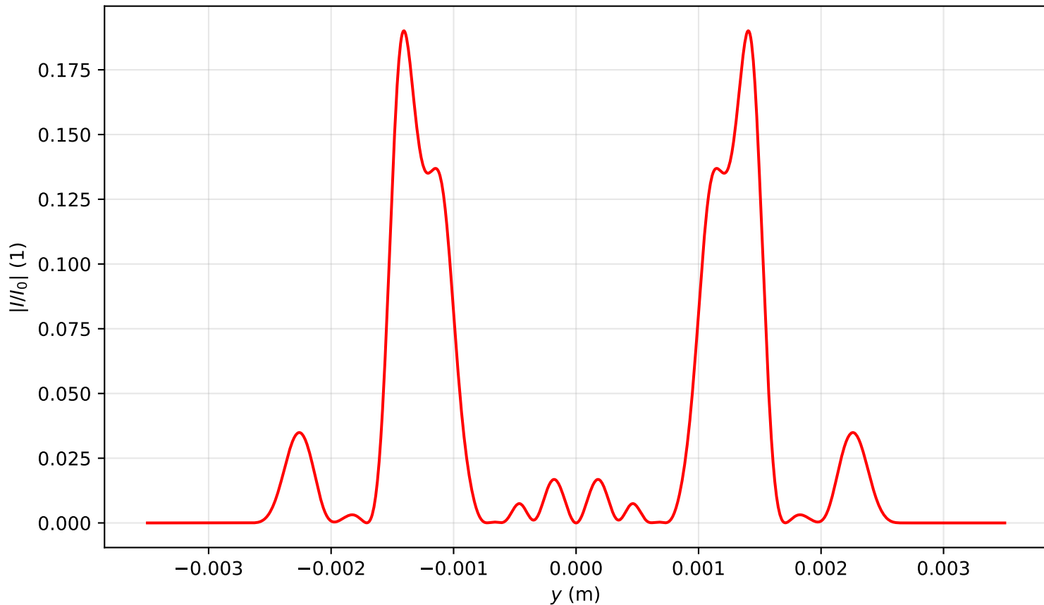
Intensity profile I(x=0, y, z=3.423)/I_0 , P_{in}=20.0\text{Pcr} , artificial time
