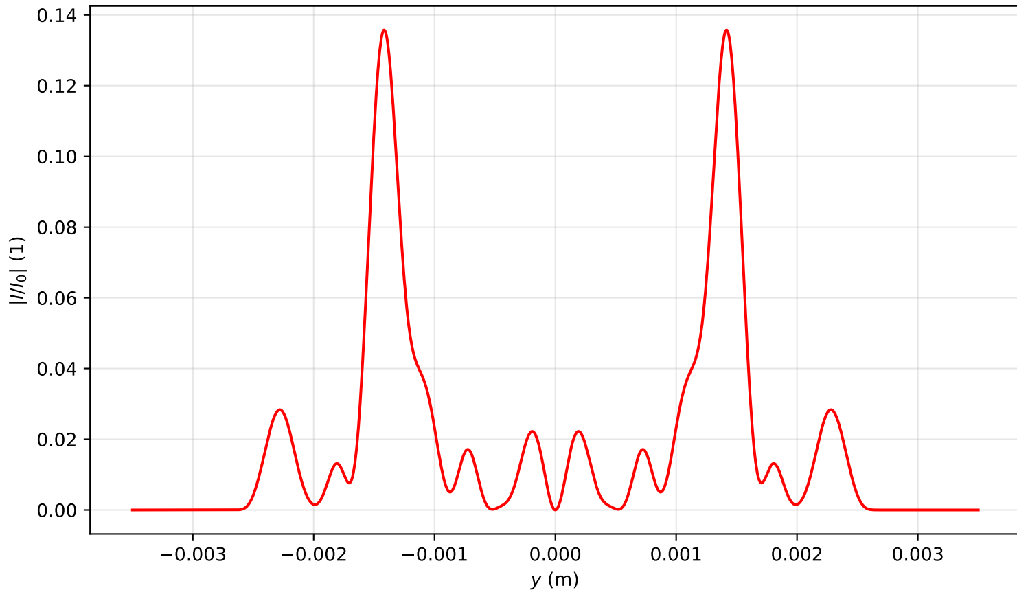
Intensity profile I(x = 0, y, z = 3.582)/I_0 , P_{in}=20.0\text{Pcr} , artificial time
