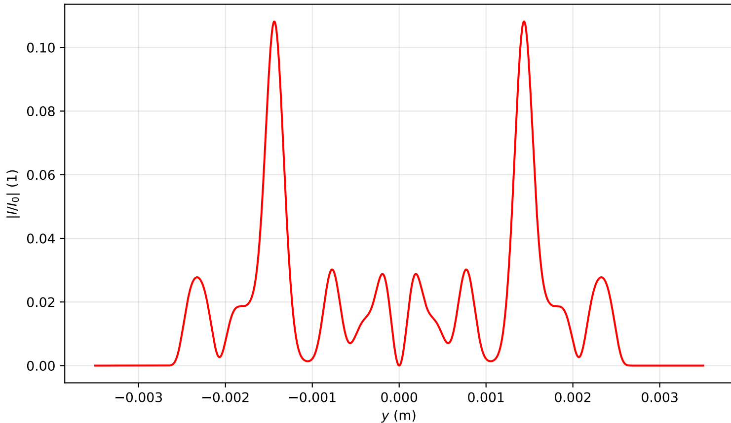
Intensity profile I(x=0, y, z=3.742)/I_0 , P_{in}=20.0\text{Pcr} , artificial time
