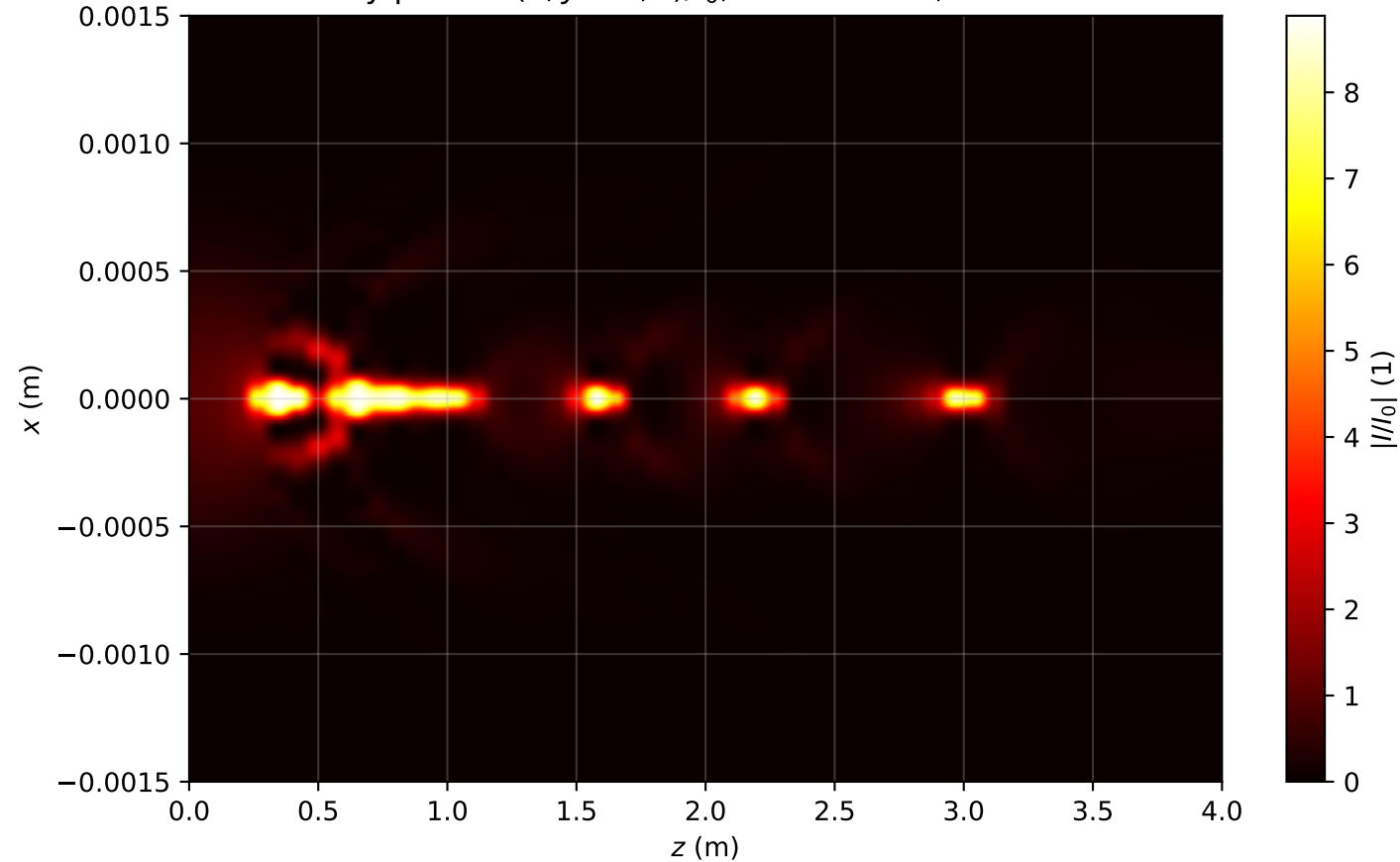
Intensity profile I(x, y = 0, z)/I_0 , P_{in}=12.5P_{cr} , artificial time
