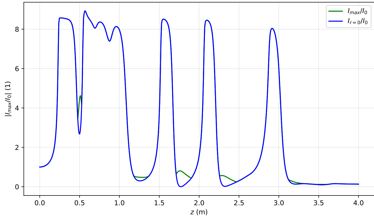
I_{max}(x=0, y=0, z)/I_0 , Pin=13.0Pcr, artificial time
