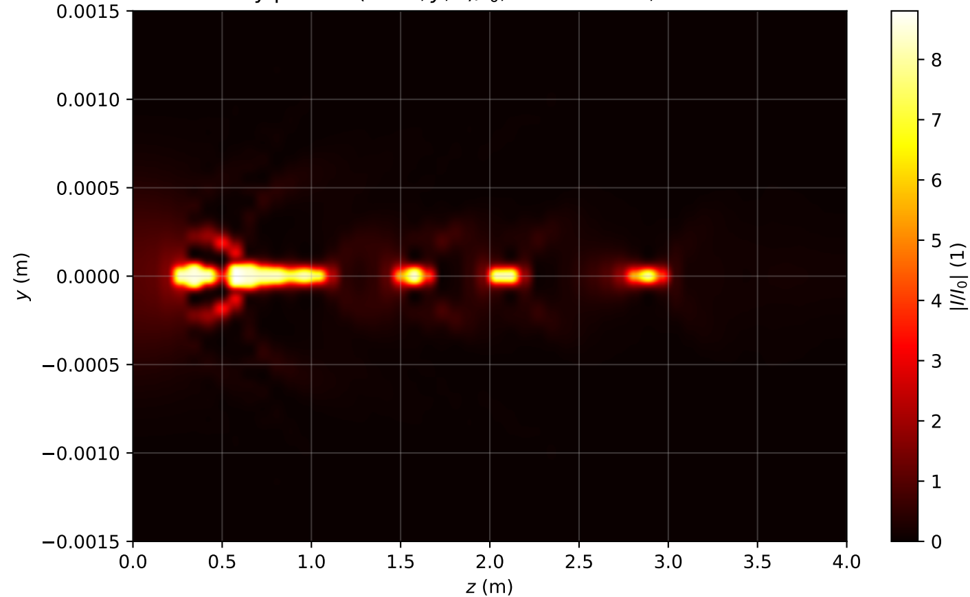
Intensity profile I(x = 0, y, z)/I_0 , P_{in}=13.0\text{Pcr} , artificial time
