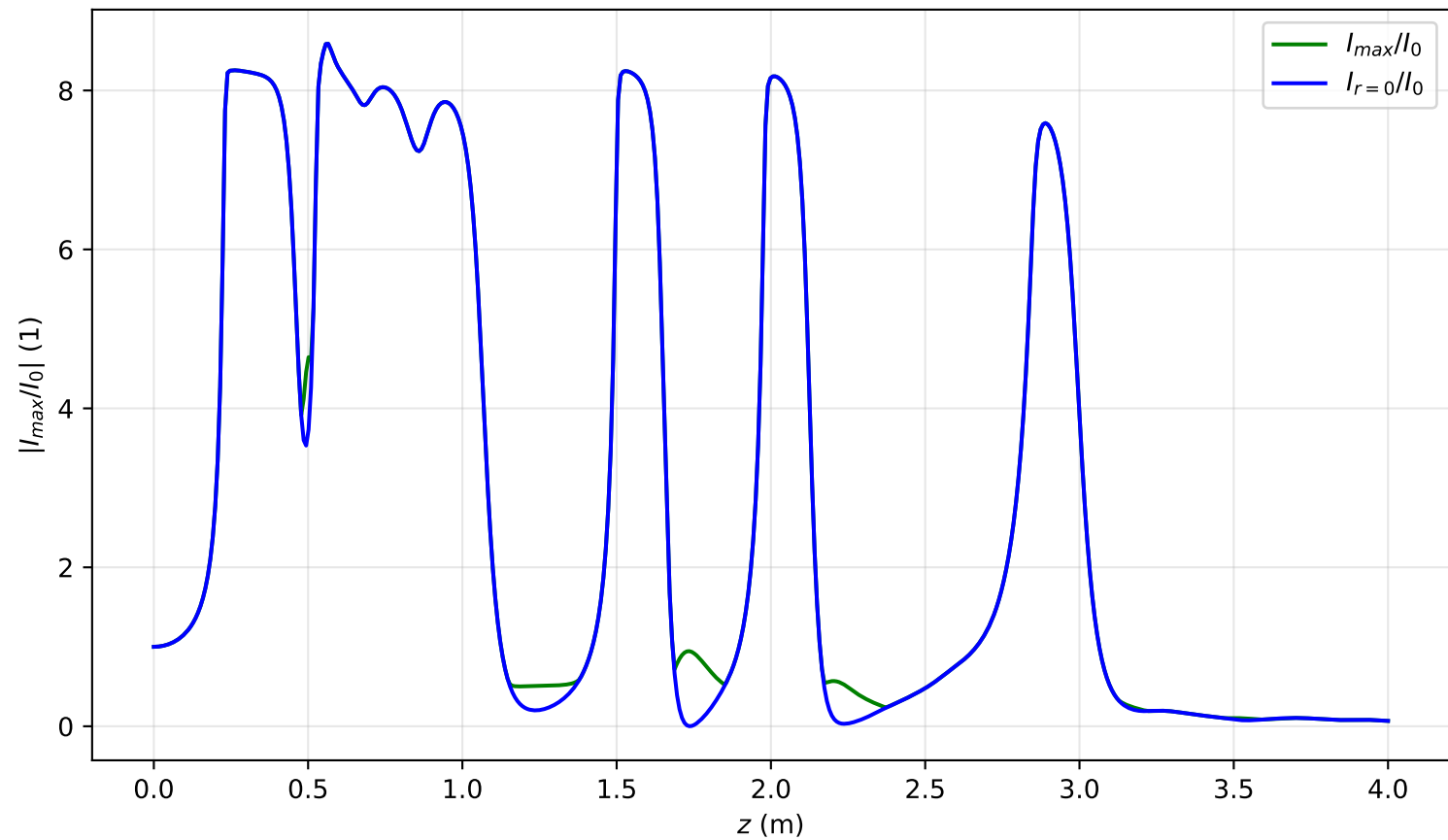
I_{max}(x = 0, y = 0, z)/I_0 , Pin=13.5Pcr, artificial time
