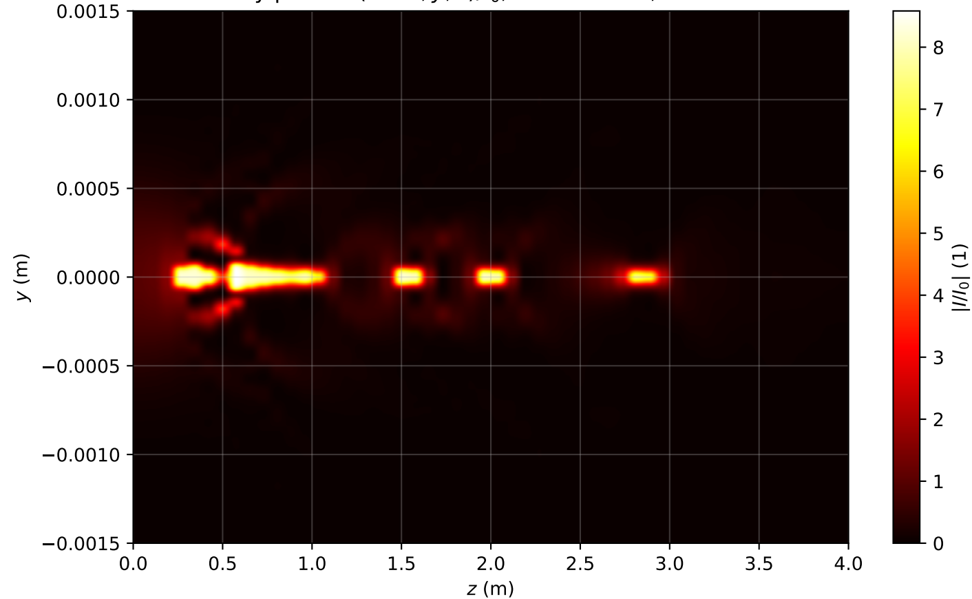
Intensity profile I(x = 0, y, z)/I_0 , P_{in}=13.5P_{cr} , artificial time
