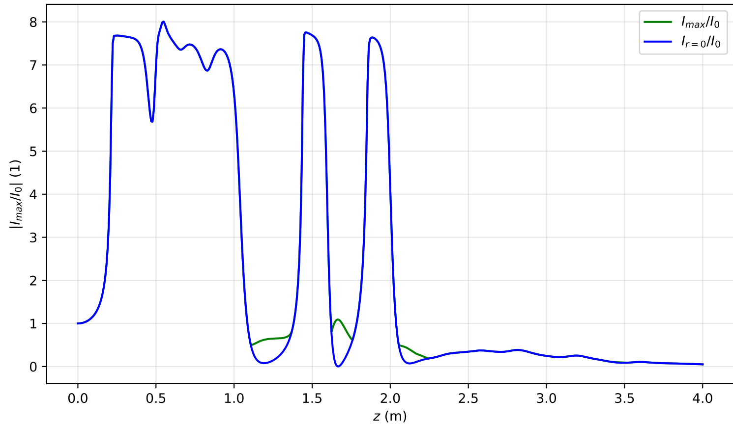
I_{max}(x = 0, y = 0, z)/I_0 , \text{Pin}=14.5\text{Pcr} , artificial time
