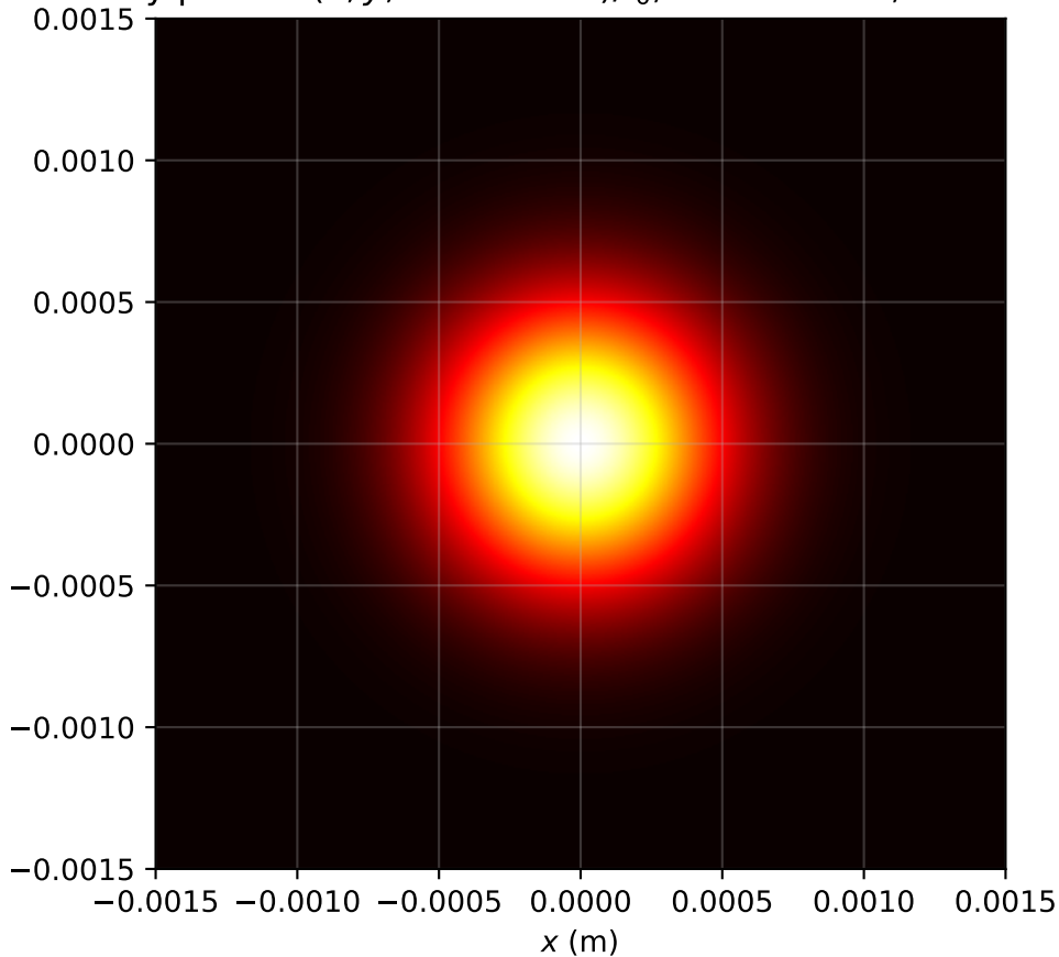
Intensity profile I(x, y, z = 0.000m)/I_0 , P_{in}=14.5P_{cr} , artificial time
