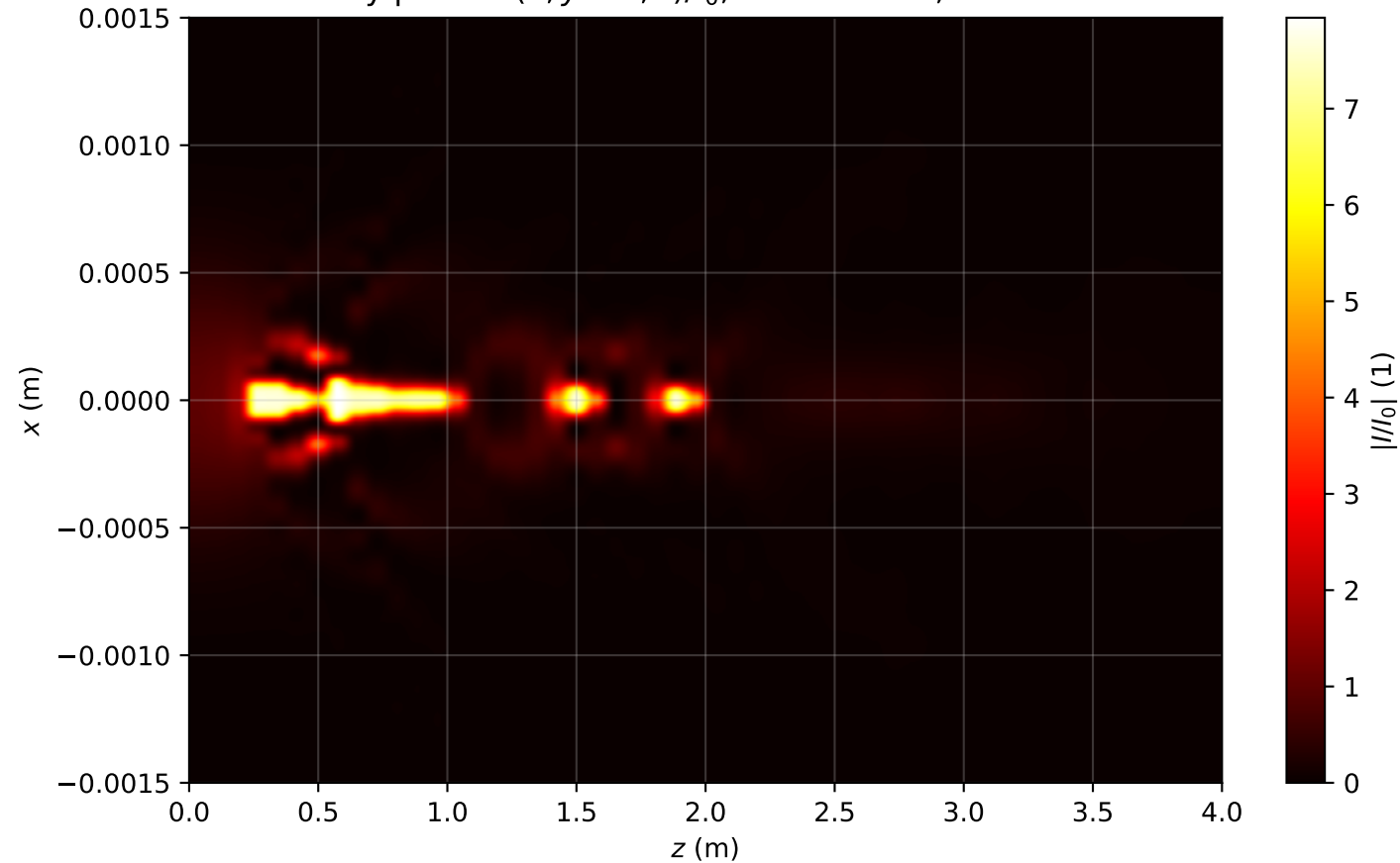
Intensity profile I(x, y = 0, z)/I_0 , P_{in}=14.5P_{cr} , artificial time
