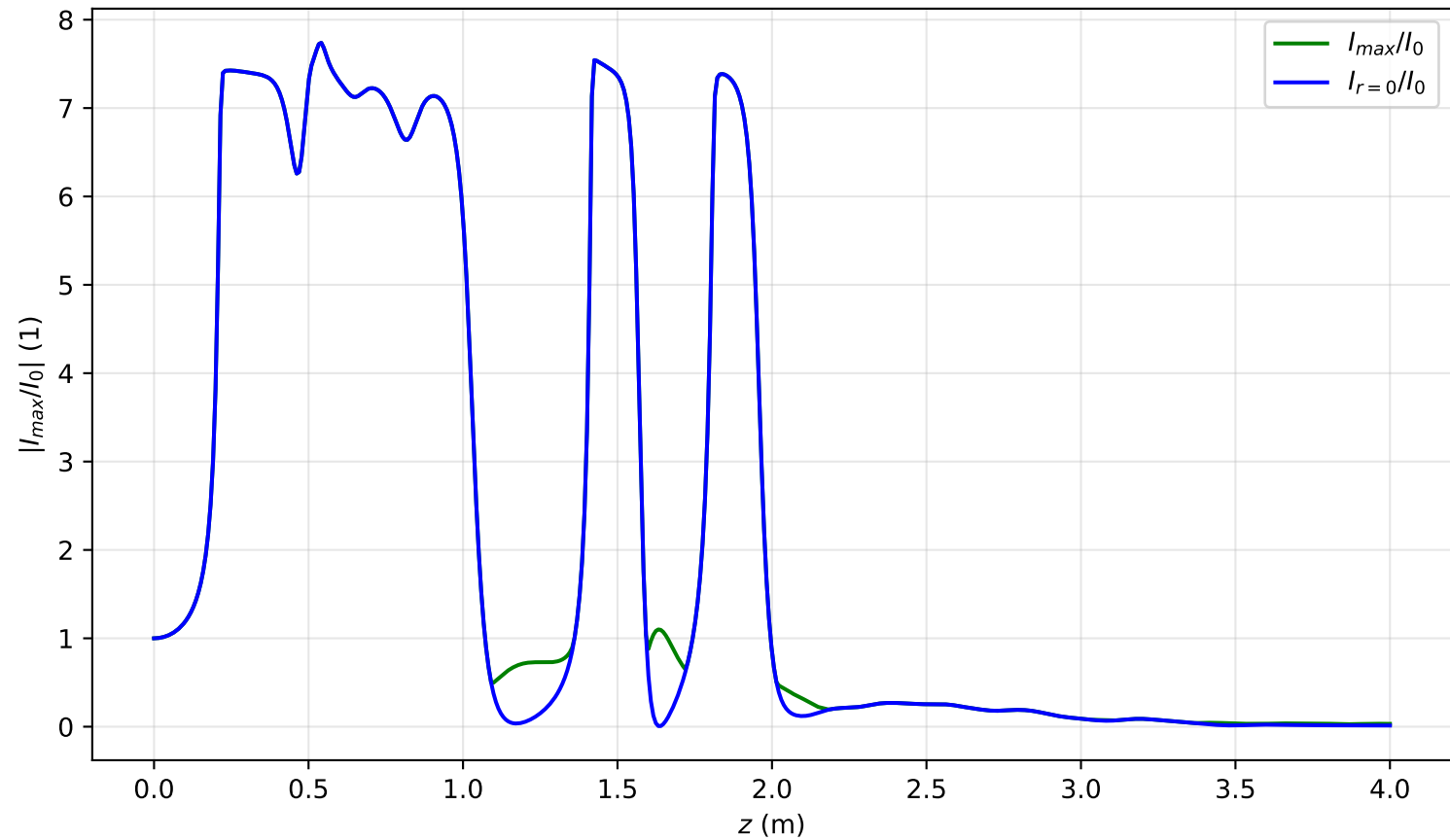
I_{max}(x = 0, y = 0, z)/I_0 , Pin=15.0Pcr, artificial time
