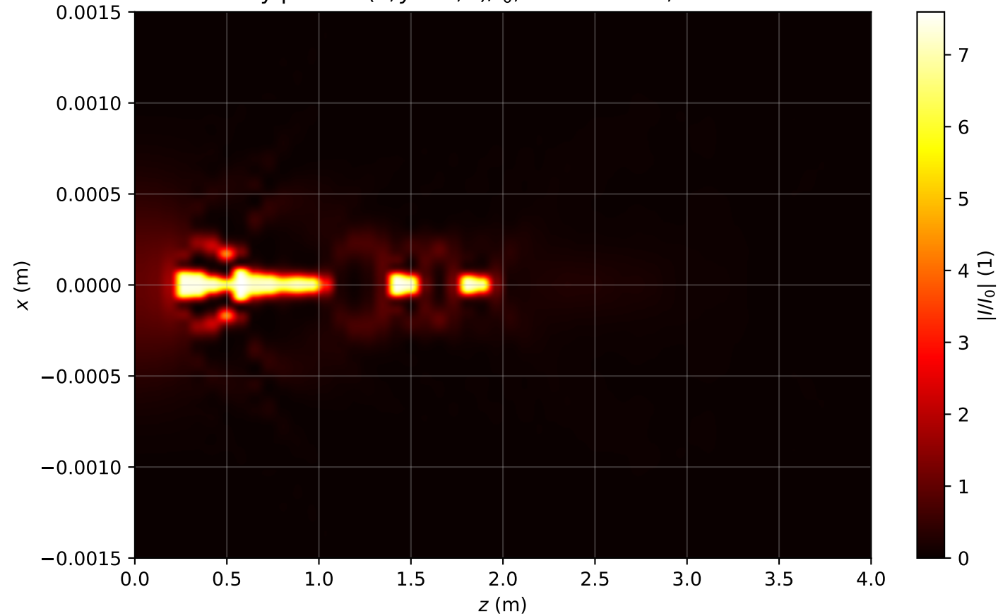
Intensity profile I(x, y = 0, z)/I_0 , P_{in}=15.0P_{cr} , artificial time
