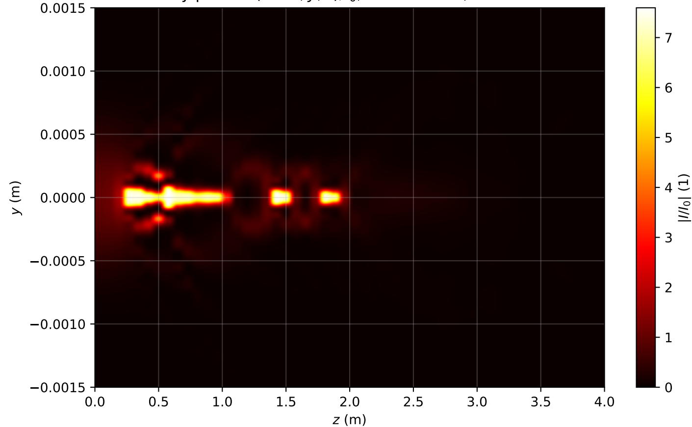
Intensity profile I(x=0, y, z)/I_0 , P_{in}=15.0P_{cr} , artificial time
