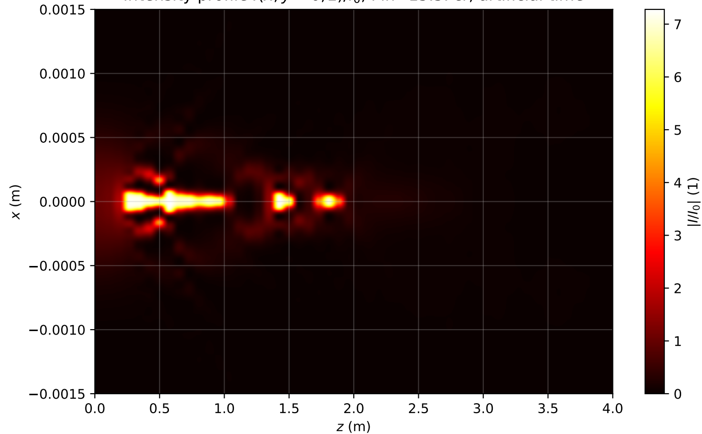
Intensity profile I(x, y = 0, z)/I_0 , P_{in}=15.5P_{cr} , artificial time
