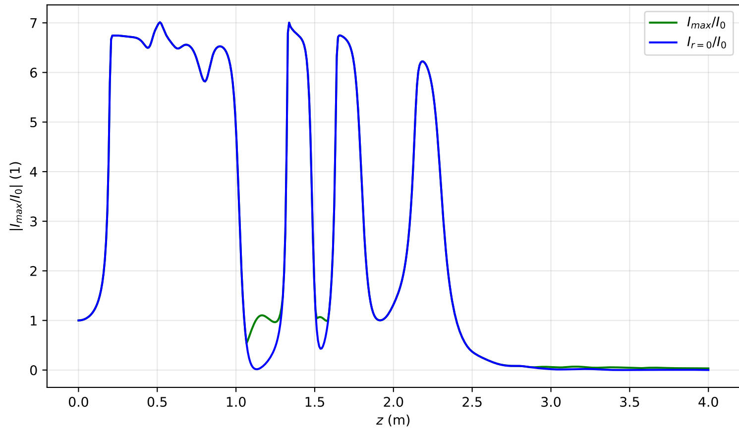
I_{max}(x = 0, y = 0, z)/I_0 , Pin=16.5Pcr, artificial time
