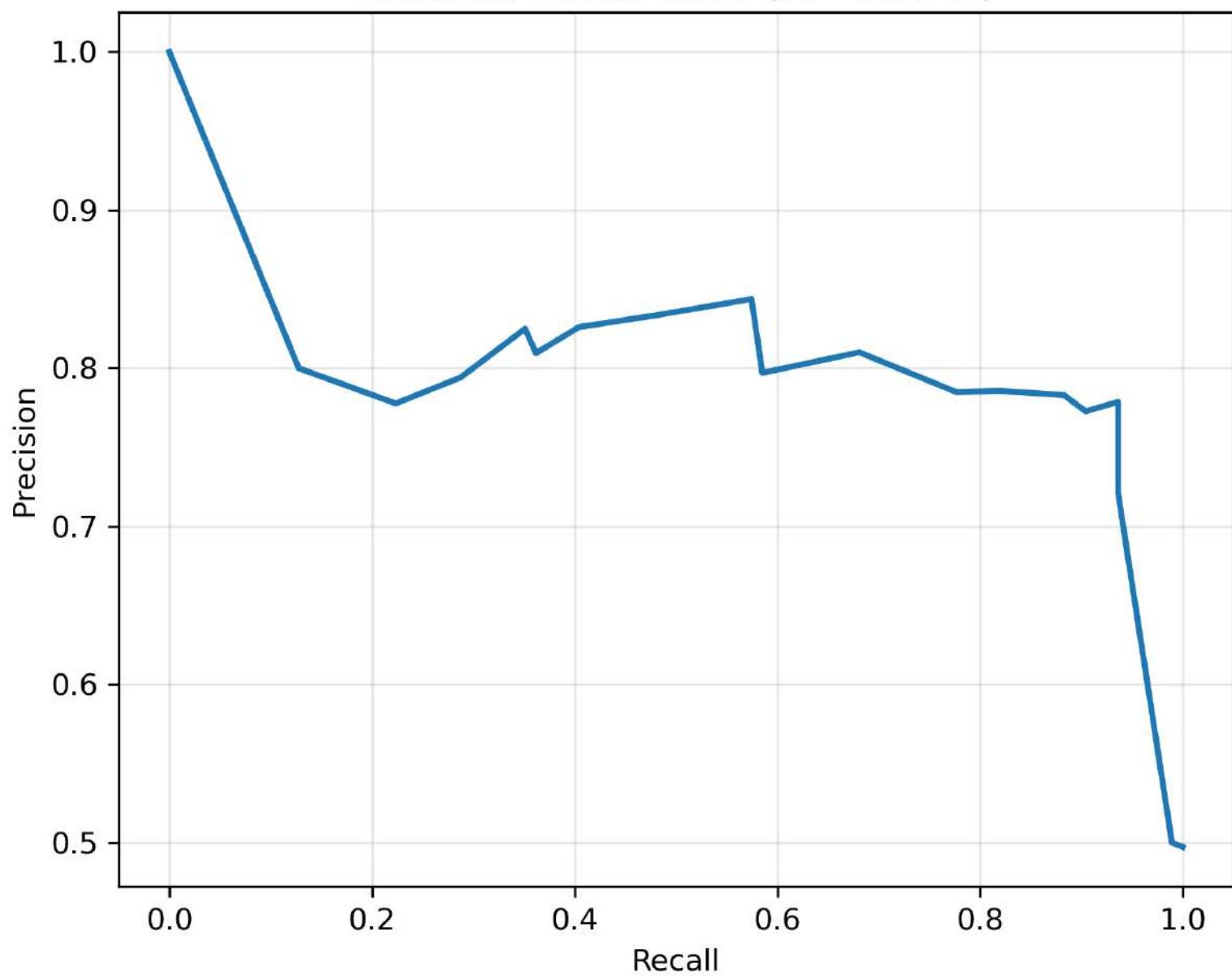
Precision-Recall Curve (AP=0.7843)
