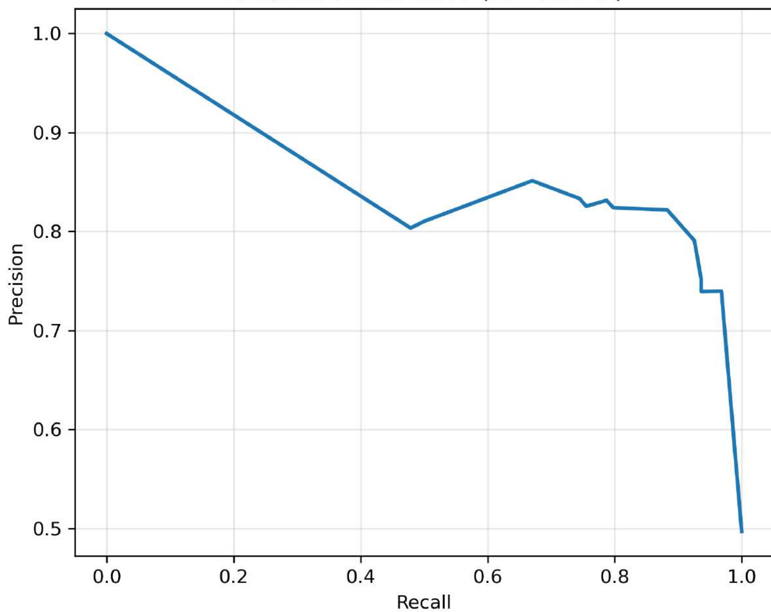
Precision-Recall Curve (AP=0.8041)
