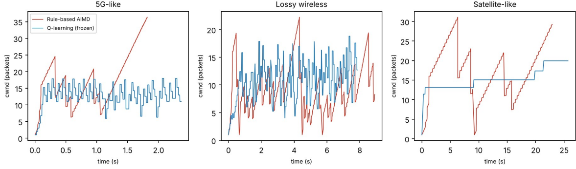
Figure 22: Congestion window over time in one evaluation run of each mode and scenario
