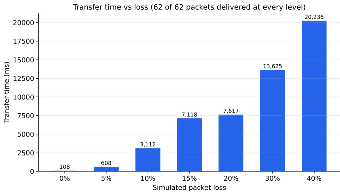
Figure 3: Transfer time against simulated loss, from the benchmark in Table 5; all 62 packets were delivered at every level
