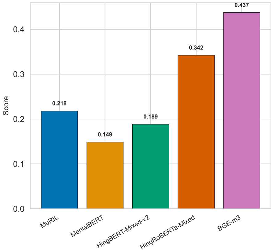
Retrieval nDCG@10
