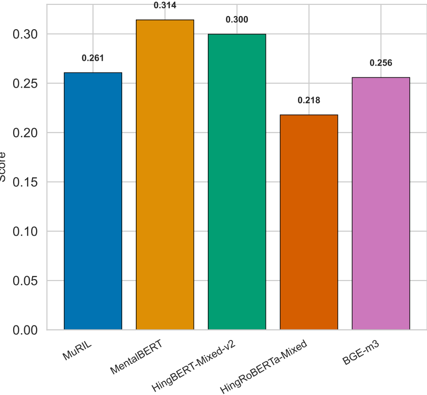
Keyword Stability
