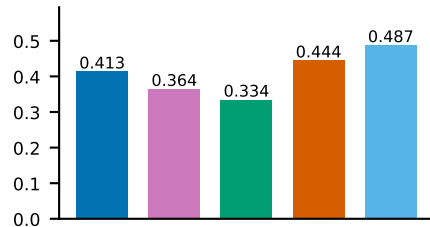
Topic diversity
