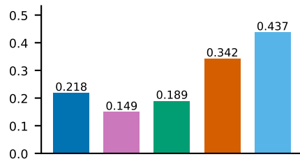
Retrieval nDCG@10
