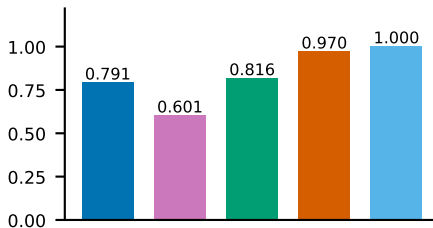
Retrieval MRR
