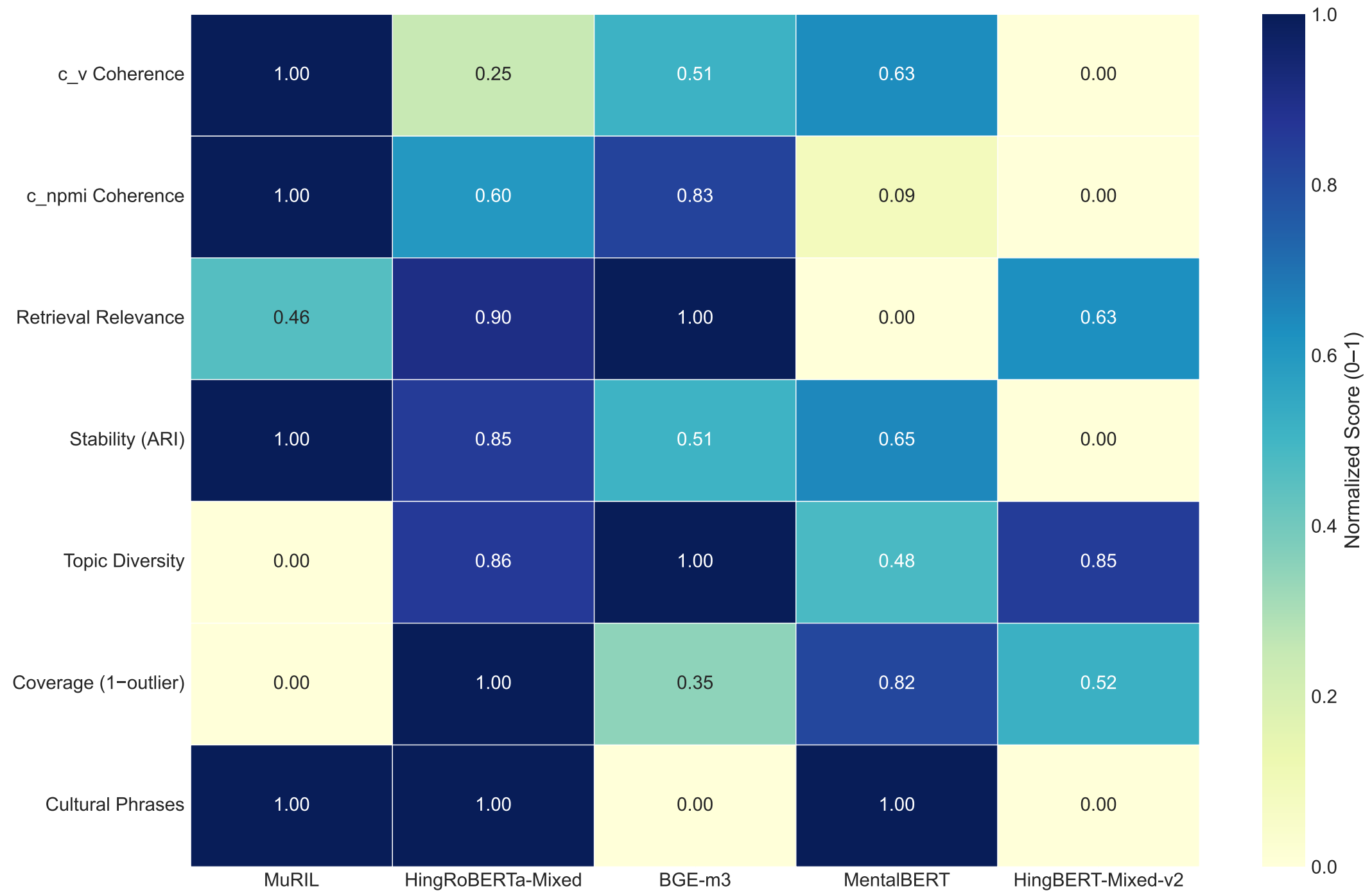
Normalized Metric Comparison: Comments Corpus (Higher = Better for All Metrics)
