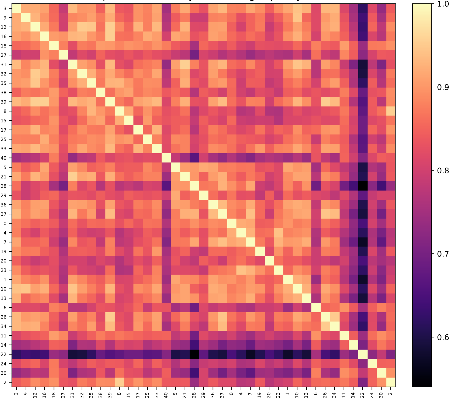
Inter-topic cosine similarity (centroids, grouped by theme)
