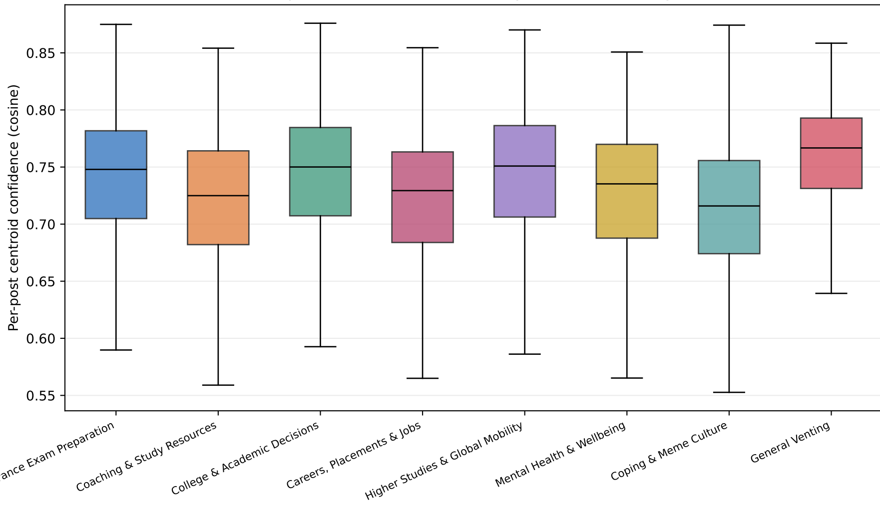
Within-topic confidence distribution by theme (cluster tightness)
