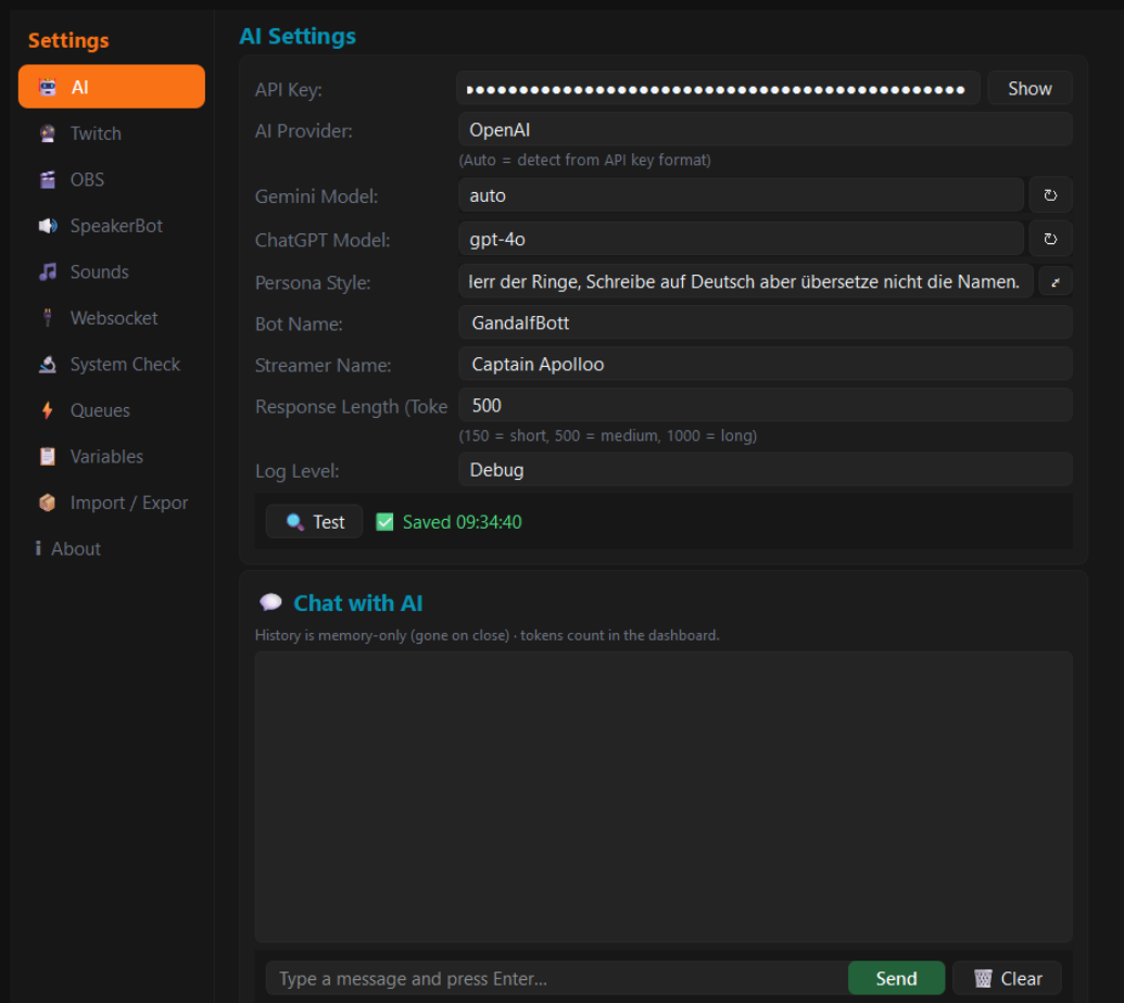
The AI settings with the chat window below
