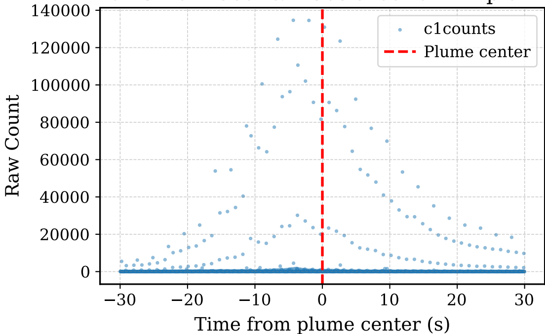
INMS Raw Count: \pm 30 s around E14 plume
