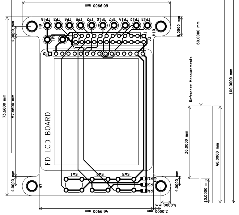
FD PCB Layouts V2 – Separated Barrel, with Peninsula
