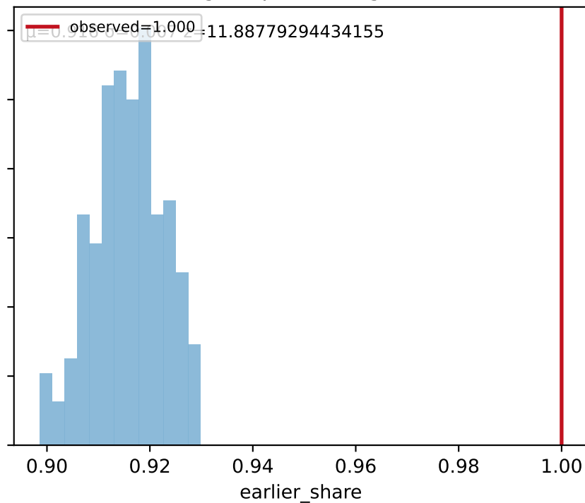
Degree-preserving null
