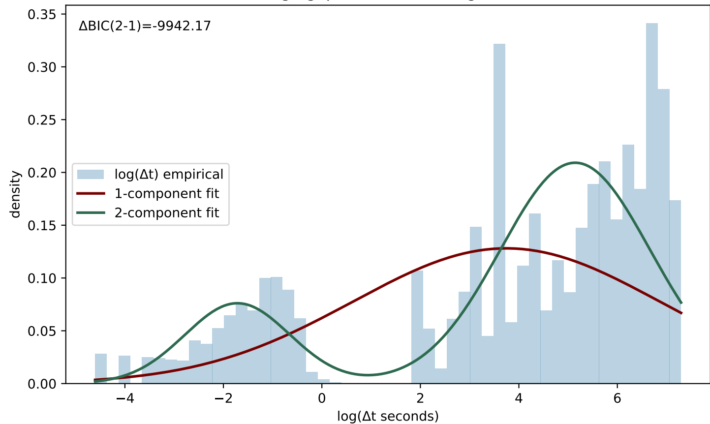
Age-gap mixture fit on \log(\Delta t)
