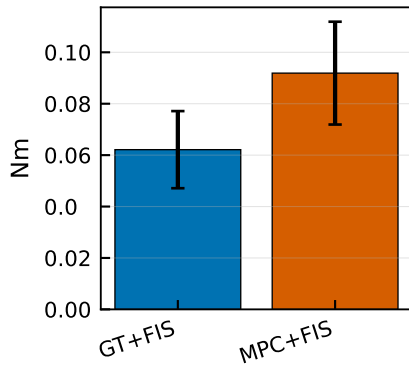
Control torque
