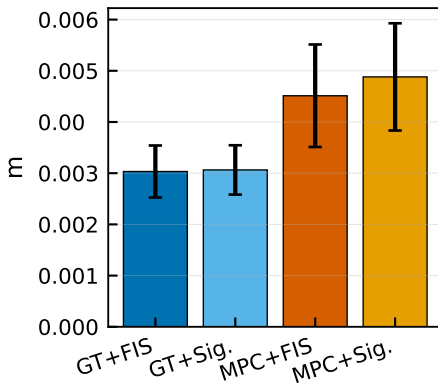
Force smoothness
