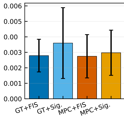
Force smoothness
