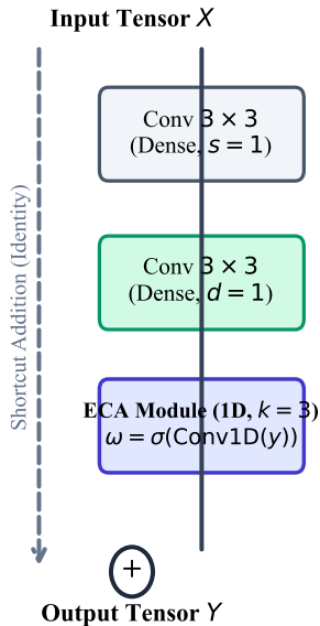
(b) Dense C2f_ECA Bottleneck (Proposed P2 & P3 Stages)
