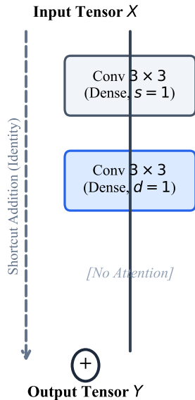
(a) Standard Bottleneck (Stock YOLOv8 Baseline)
