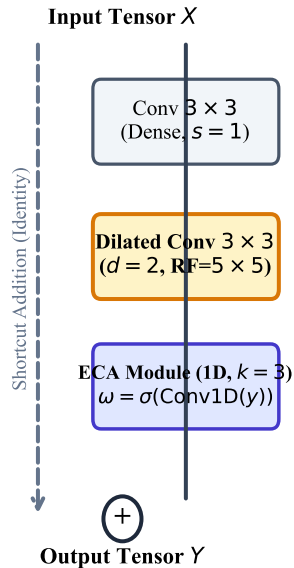
(c) Dilated C2f_ECA Bottleneck (Proposed P4 & P5 Stages)
