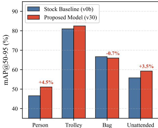
(b) Localization Precision (mAP@50-95)
