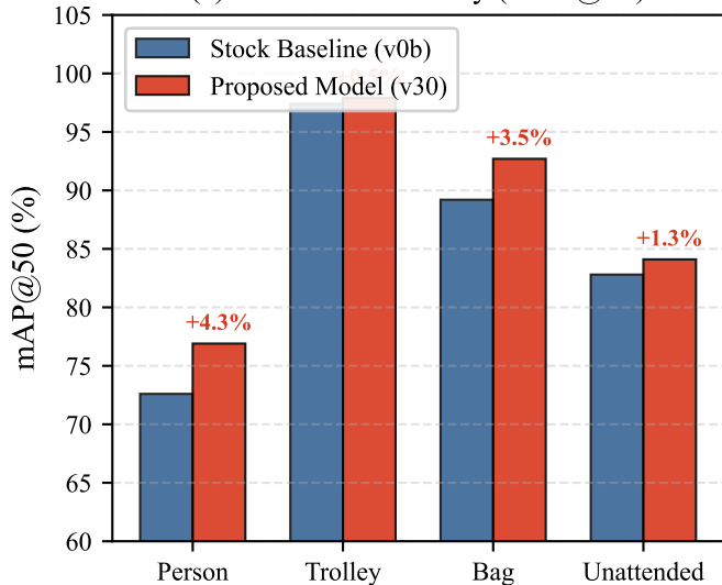
(a) Detection Accuracy (mAP@50)
