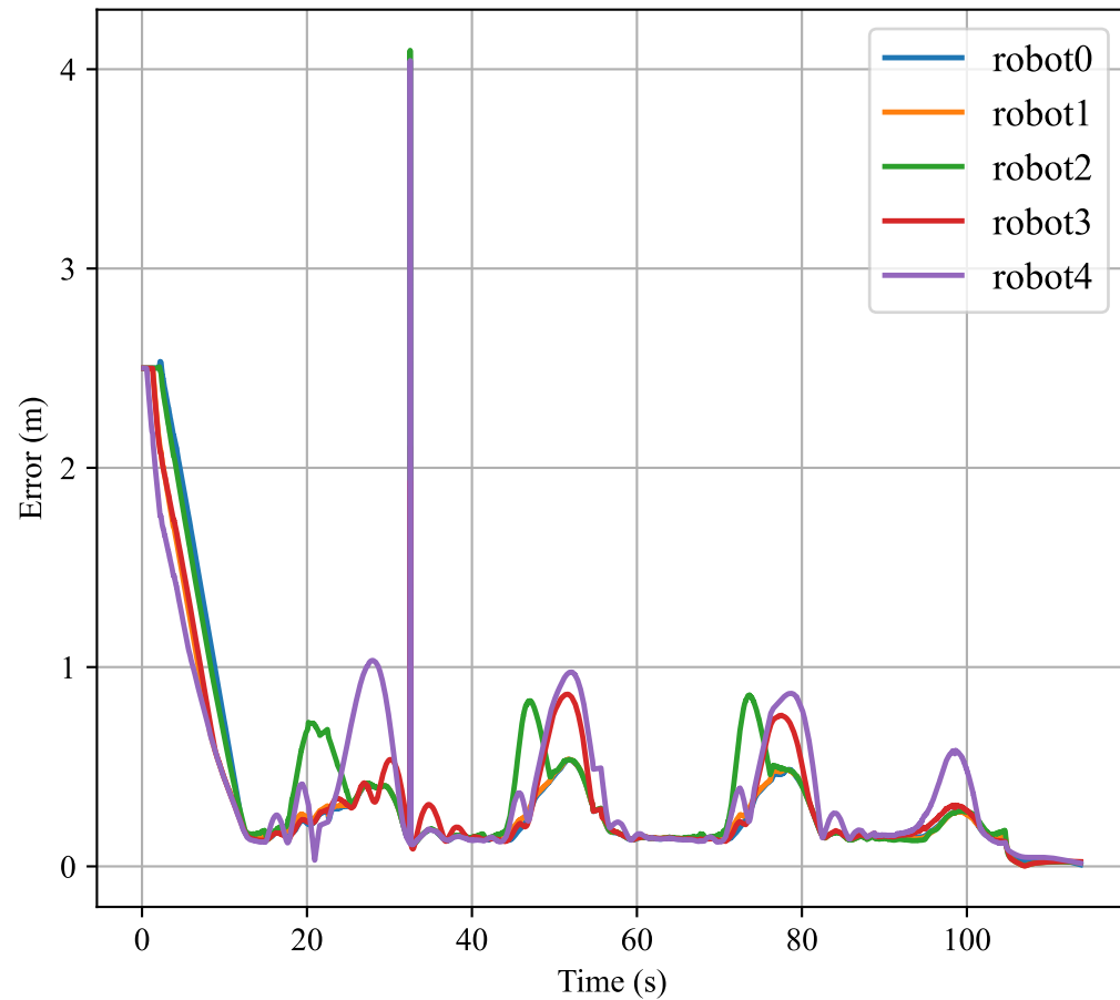
Formation error evolution
